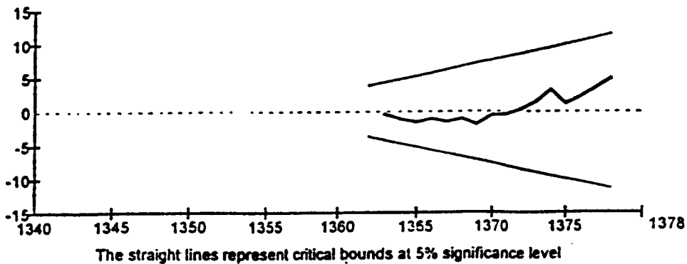
Plot of Cumulative Sum of Recursive Residuals
